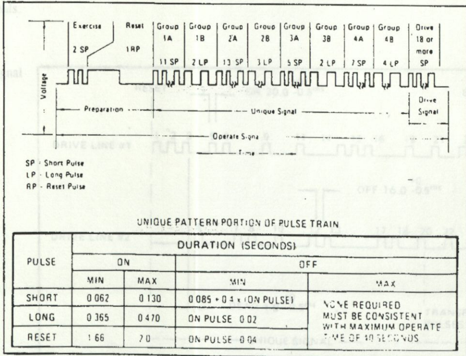
Figure 8. Intent Unique Signal (IUQS)
